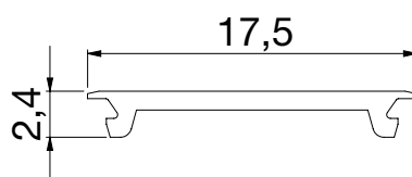
Letev YX01
