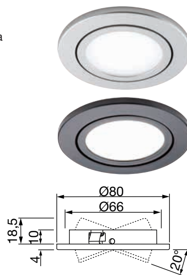
Orbit D-Motion
