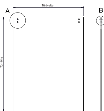
steklena drsna vrata DETAIL B
